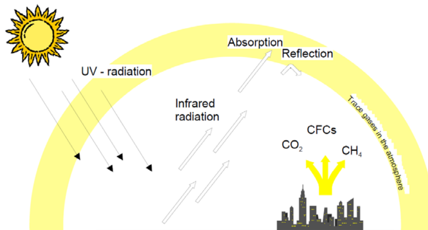
Figure 51. Greenhouse Effect
